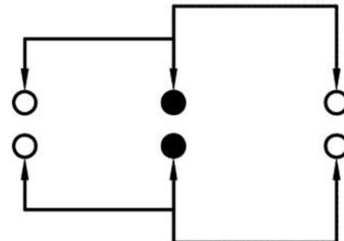
SCHEMATIC (SHORTING)
